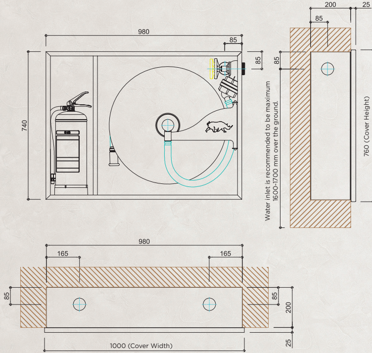
RECESSED TYPE
