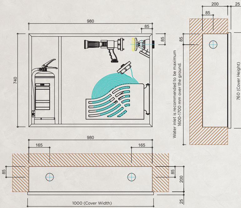
RECESSED TYPE
