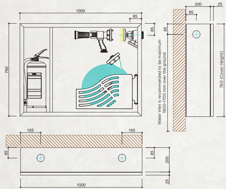
SURFACE MOUNTED TYPE
