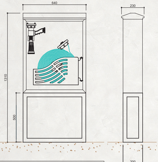
STAND MOUNTING MEASURES
