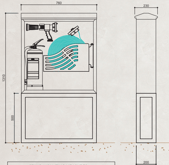
STAND MOUNTING MEASURES
